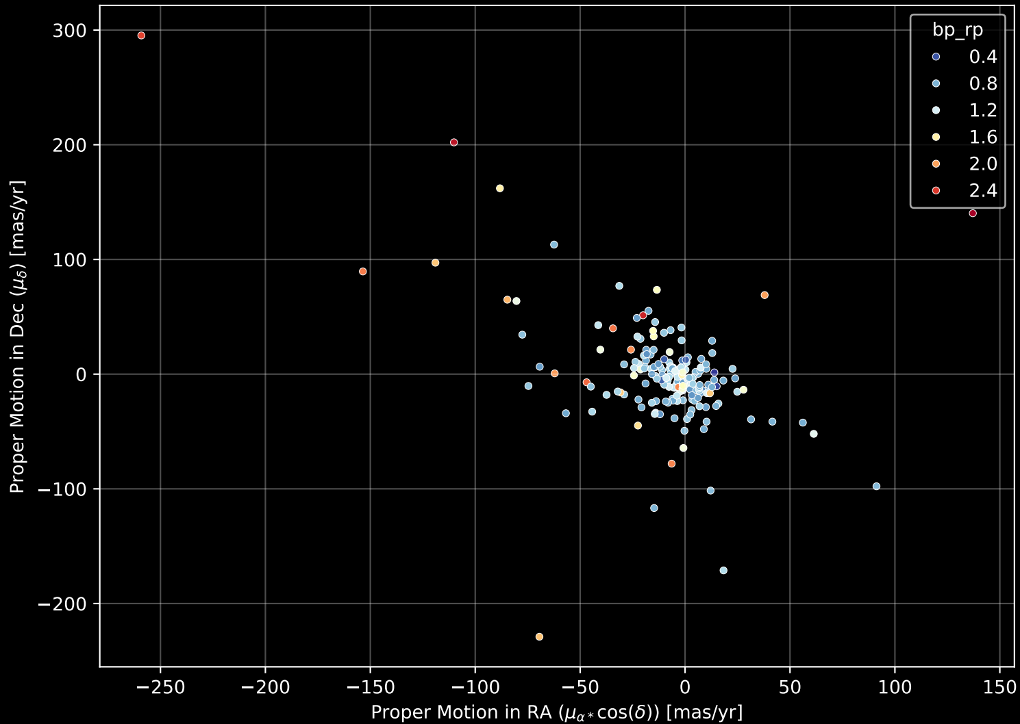
APOGEE DR17 Field: [062+45_MGA] Proper Motion Diagram (n= 193)
