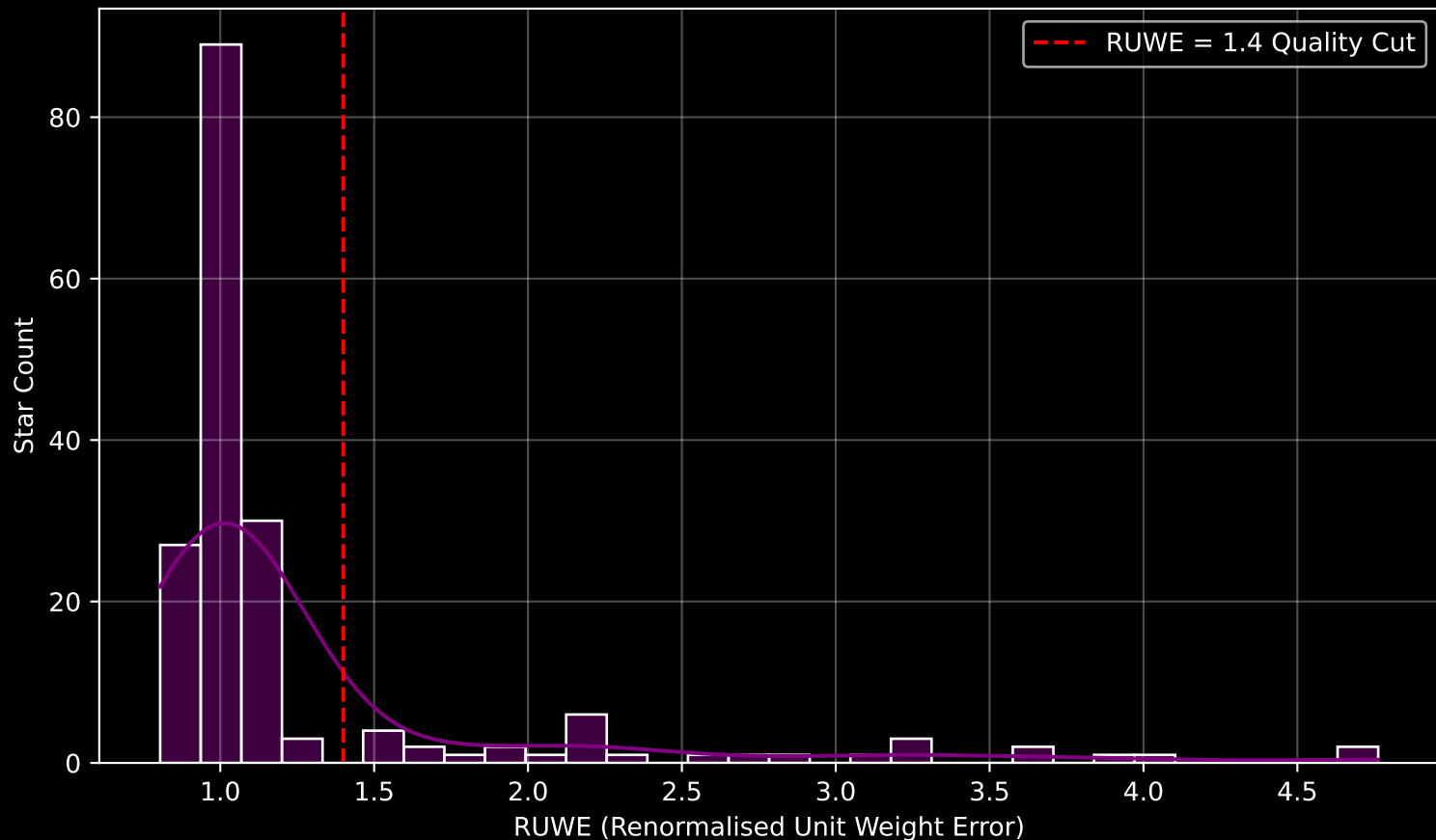
GAPOGEE DR17 Field [062+45_MGA] RUWE Distribution (n= 179)
