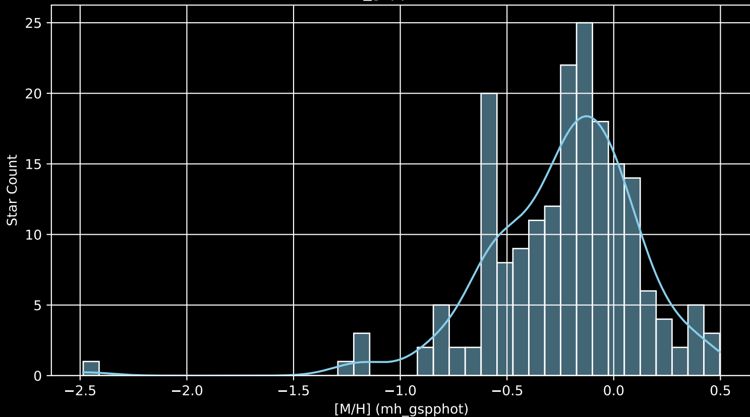
APOGEE DR17 Field: [062+45_MGA [M/H] (mh_gspphot) (n= 190)
