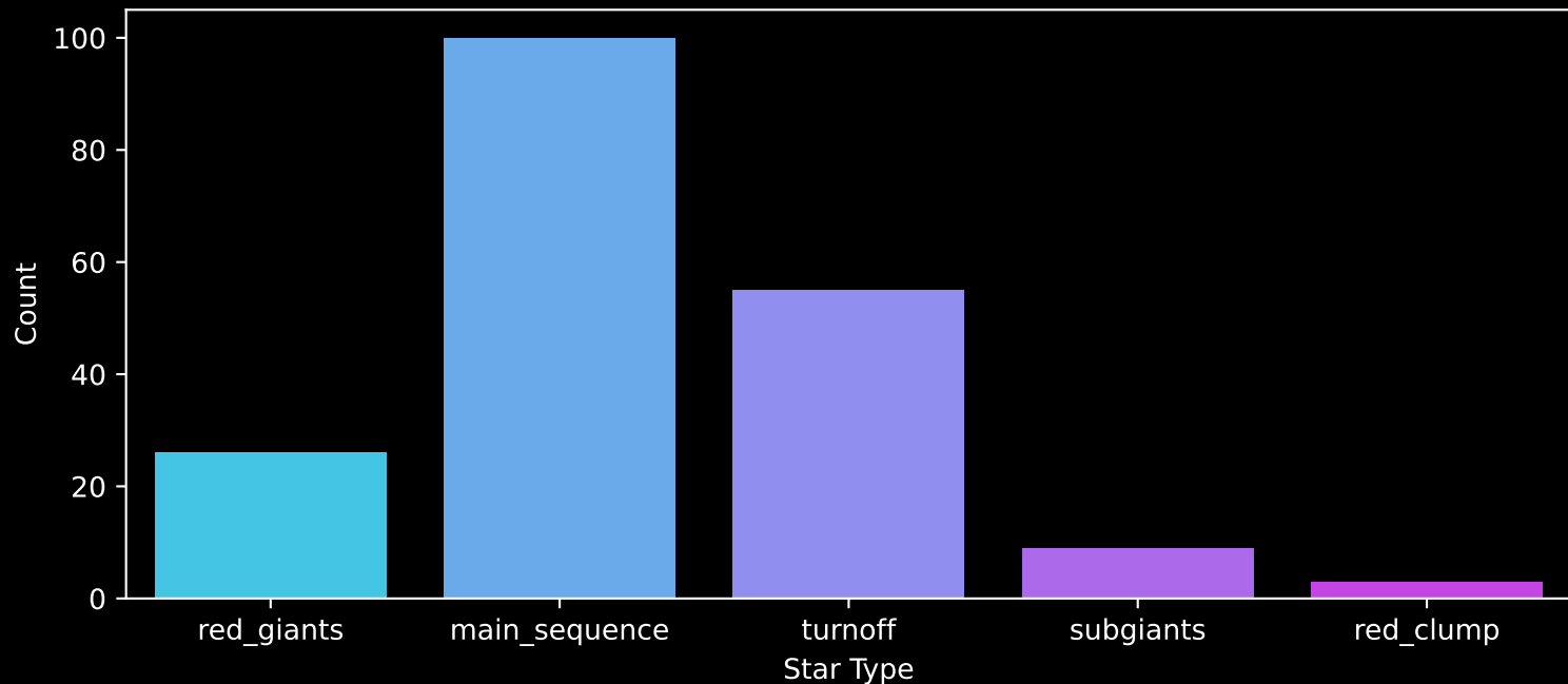
APOGEE DR17 Field: [062+45_MGA] Count plot of Star Type
