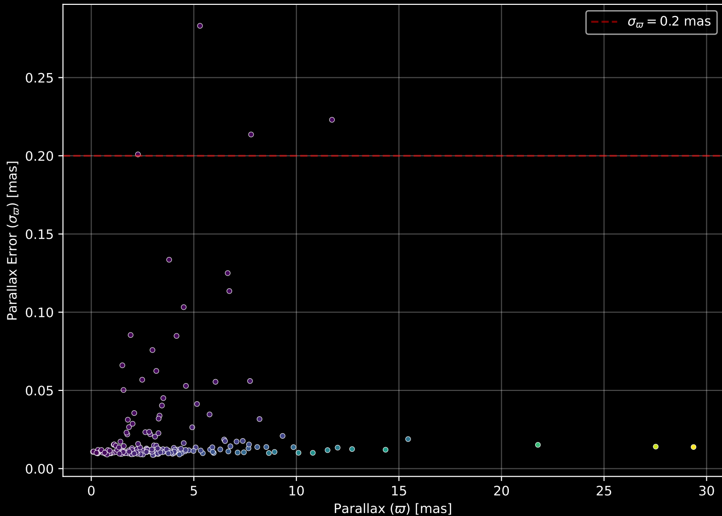
APOGEE DR17 Field: [062+45_MGA] Parallax Quality (n= 193)
