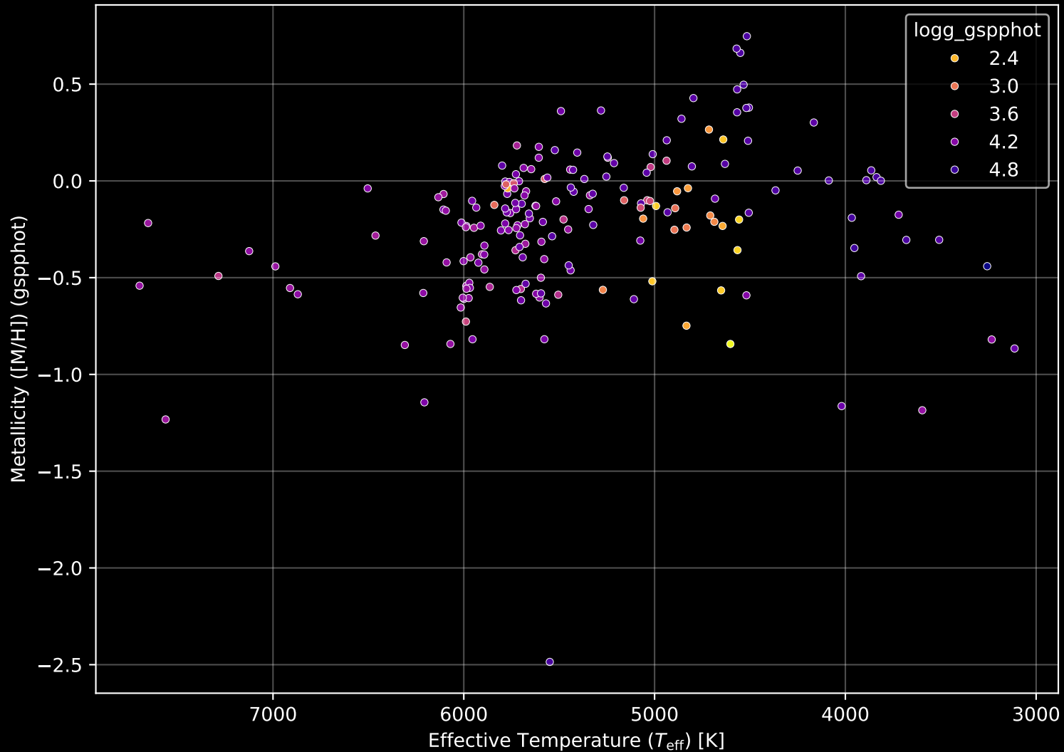
APOGEE DR17 Field: [062+45_MGA] Stellar Population Parameters (n= 193)
